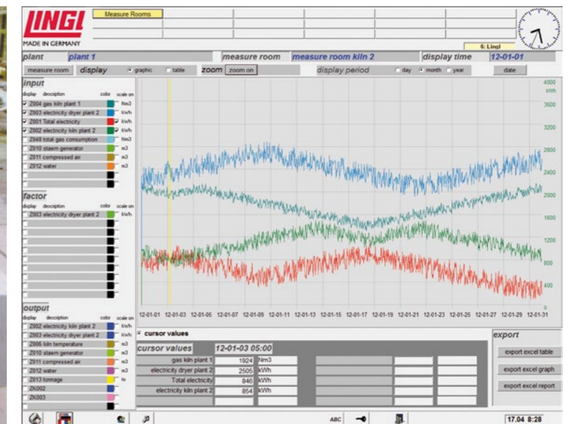
Energie-Monitoring-System Energy-Monitoring-System
